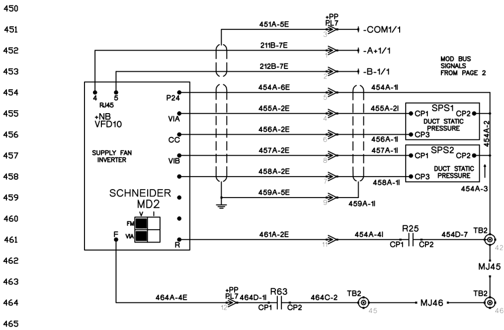
Figure 32: Schneider VFD Wiring
