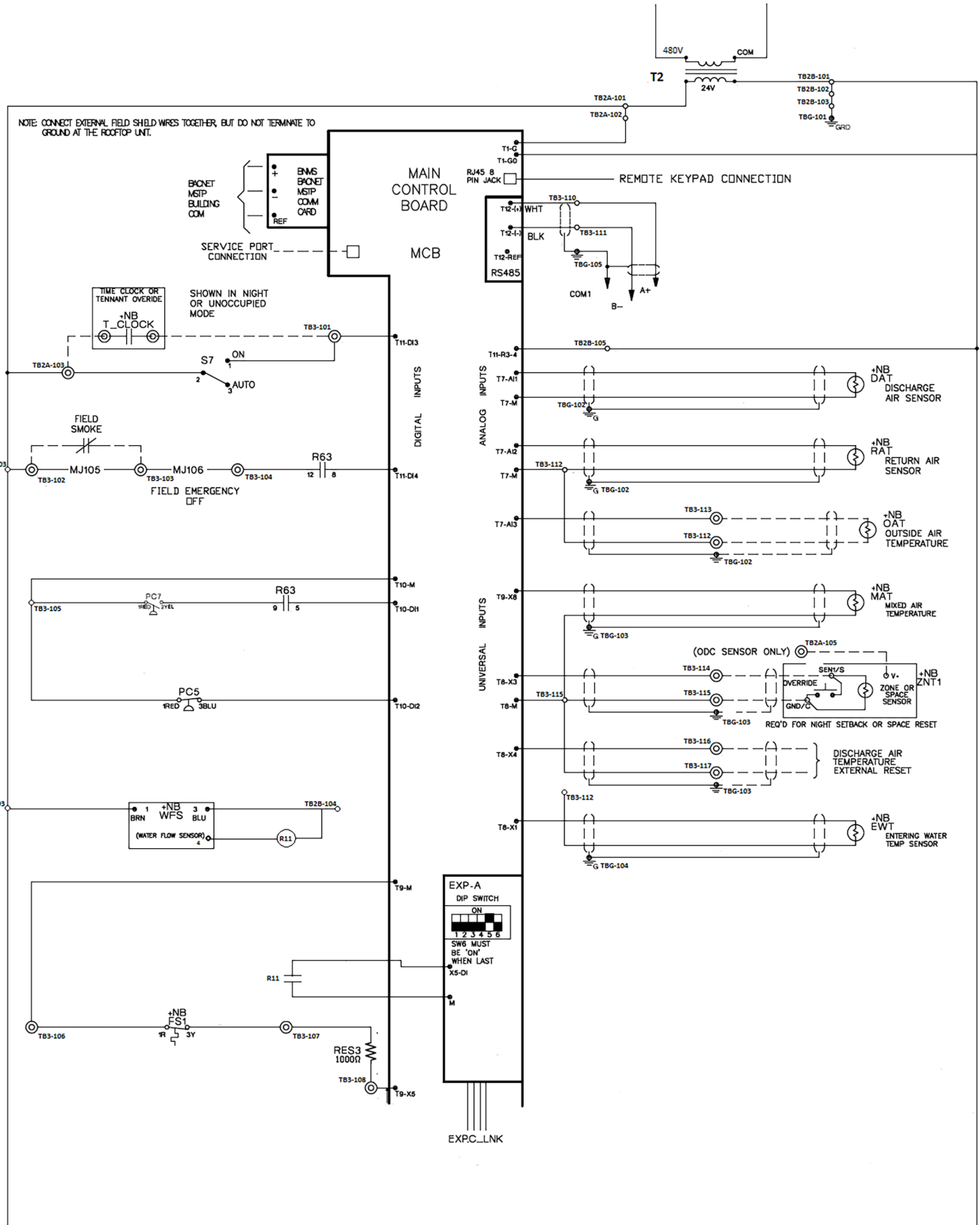
Figure 26: 200s Wiring Diagram
