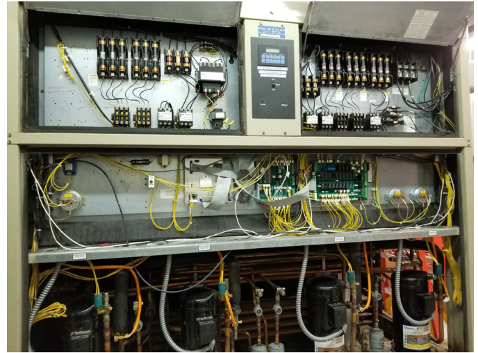
Figure 2: Main Control Board (MCB)
